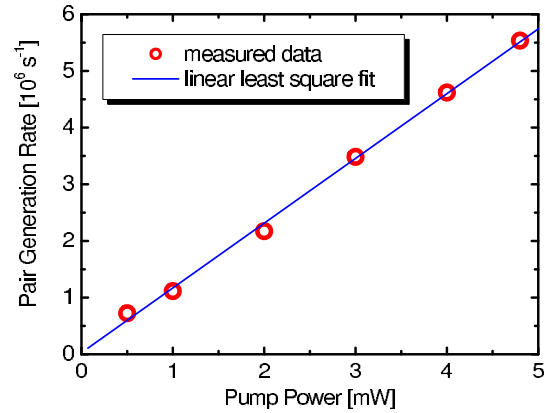
Fig. 6. Photon pair generation rate (determined from coincidence measurement) versus pump power. The symbols show the measured data, the solid line is a linear least square fit.
