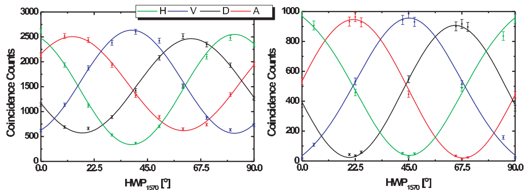
Fig. 8. Measured visibilities of the entangled photon pair source in the various bases: Left: Visibilities without the additional bandpass filter in the analysis arm and at an input pump power of 16 mW; right: visibilities with additional bandpass filter and input pump power of 6 mW.
