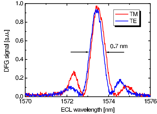
Fig. 5. Measured difference frequency power as function of the wavelength of the ECL acting as signal source for the DFG process. By setting the input polarization either to TE or TM, the two different nonlinear process can be probed separately.
