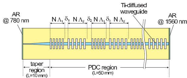
Fig. 2. Detailed design of the integrated PDC source with interlaced poling pattern.
