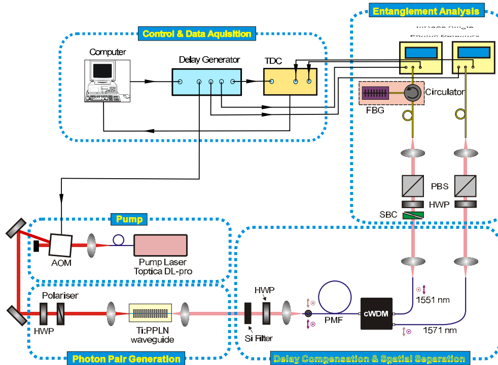
Fig. 7. Experimental setup for the investigation of entanglement. (TDC: time-to-digital converter; AOM: acoustooptical modulator; HWP: half-wave retardation plate; PMF: polarisation-maintaining fiber; cWDM: coarse WDM fiber demultiplexer; SBC: Soleil-Babinet compensator; PBS: polarisation beam splitter; FBG: fiber Bragg grating).
