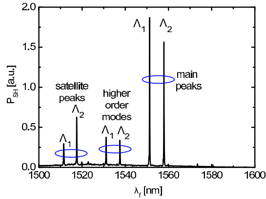
Fig. 3. Measured second harmonic power versus wavelength of the fundamental wave. Details are described in the text.
