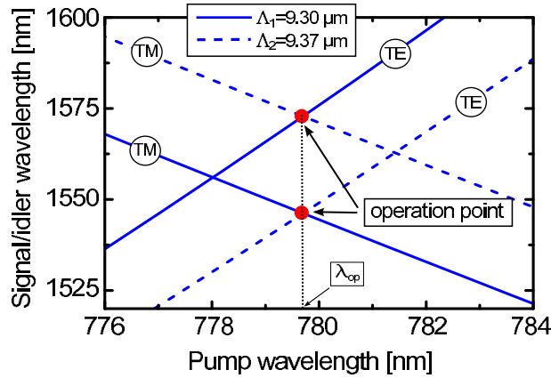
Fig. 1. Calculated phase-matching characteristics of type II phase-matched PDC processes in a PPLN waveguide assuming a poling period of \Lambda_1 = 9.30 \mu\text{m} (solid lines) and \Lambda_2 = 9.37 \mu\text{m} (dashed curves), respectively. The operation point for the generation of polarization entangled pairs is at the intersection of the phase-matching characteristics of the two periodicities.
