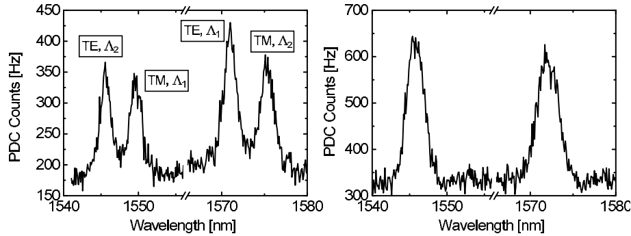
Fig. 4. Results of spectrally resolved PDC measurements with \lambda_p = 780.0 nm. Left: PDC spectrum at a sample temperature of T = 159.2 °C resulting in separated spectral peaks. Right: Same measurement at T = 156.4 °C indicating the correct operation point for polarization entanglement.
